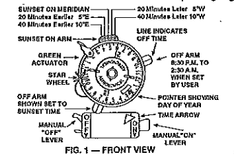
FIG. 1 - FRONT VIEW
