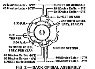
FIG. 2 - BACK OF DIAL ASSEMBLY
