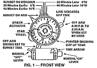
FIG. 1 - FRONT VIEW
