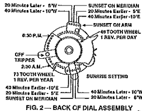
FIG. 2 - BACK OF DIAL ASSEMBLY
