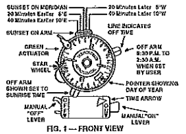
FIG. 1 - FRONT VIEW
