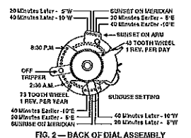
FIG. 2 - BACK OF DIAL ASSEMBLY
