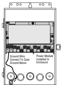
POWER MODULE (front view)
