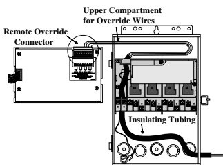
REMOTE OVERRIDE WIRING
