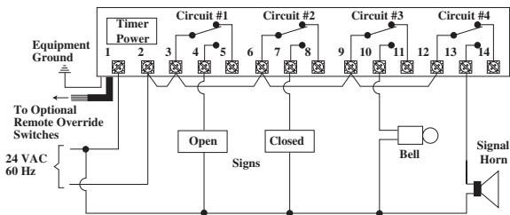
Example #1: All loads and timer powered by same source
