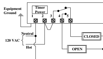
ET701I5C SPDT 120 Volt Input Alternating Sign Control / Fixed Switching
