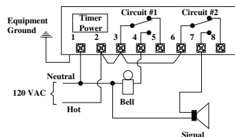
ET702I5C 2-SPDT 120 Volt Input Bell and Signal Controls / Pulse and Interval Switching (Loads and Timer Powered by Same Source)
