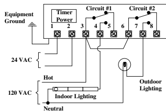
ET70215CR24 2-SPDT 24 Volt Input Indoor and Outdoor Lighting / Astro Switching Circuit #2 Only (Loads and Timer Each Powered by Different Sources and Voltages)
