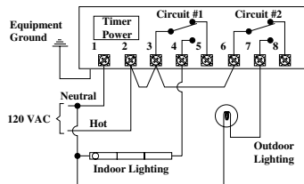
ET702I5C 2-SPDT 120 Volt Input Indoor and Outdoor Lighting / Astro Switching Circuit #2 Only
